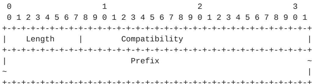
Figure 3: NLRI For Withdrawal
