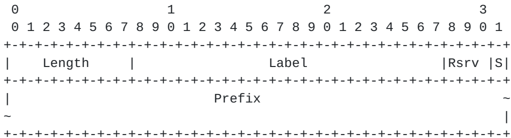
Figure 1: NLRI With One Label
