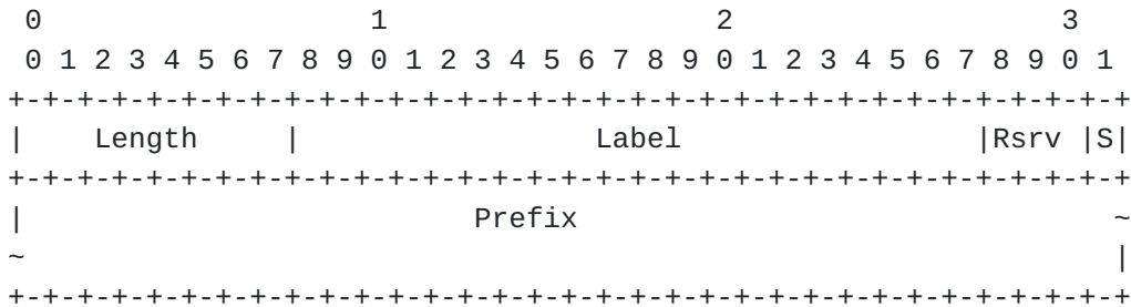
Figure 2: NLRI With One Label
