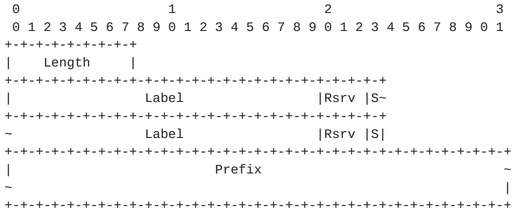
Figure 3: NLRI With Multiple Labels
