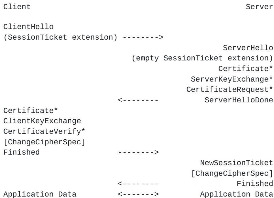
Figure 4: Message flow for server rejecting ticket, performing full handshake and issuing new session ticket
