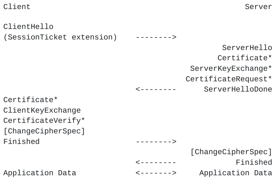
Figure 3: Message flow for server completing full handshake without issuing new session ticket
