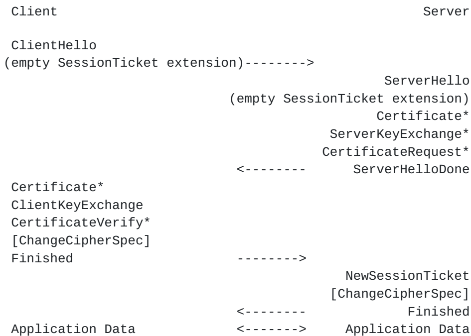
Figure 1: Message flow for full handshake issuing new session ticket
