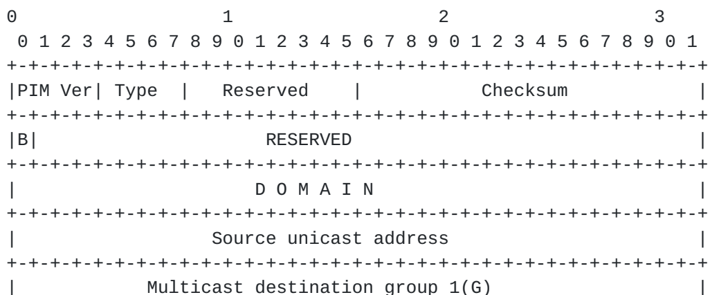
Figure 2 source register request packet
