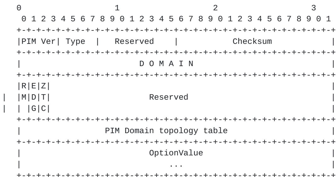
Figure 23 hello packet containing RP address
