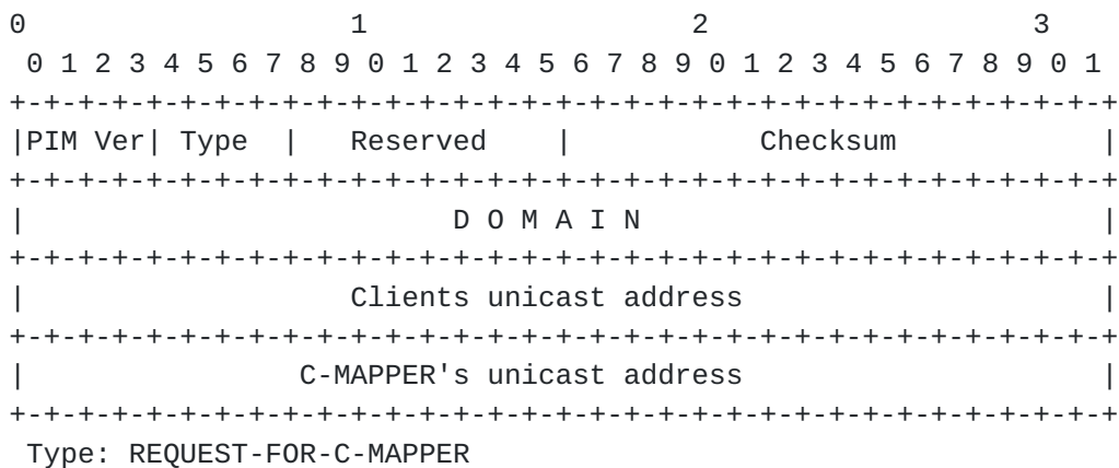
Figure 22 request- for-C-MAPPER packet sent to the SC-MAPPER
