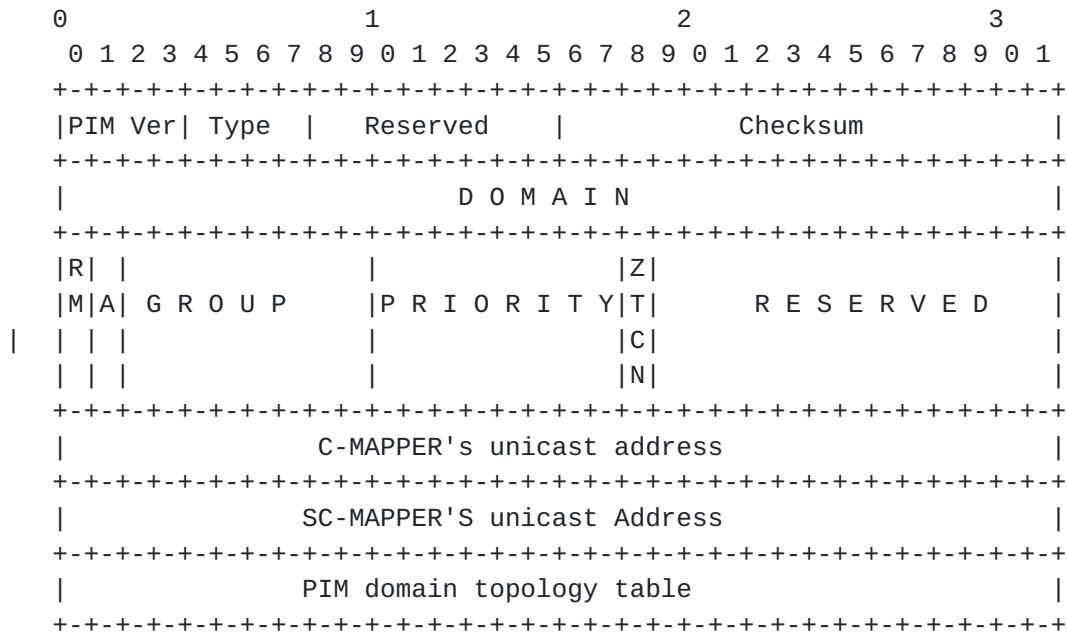
Figure 17 SC-MAPPER/RP answers to a host REQUEST-FOR-C-MAPPER message
