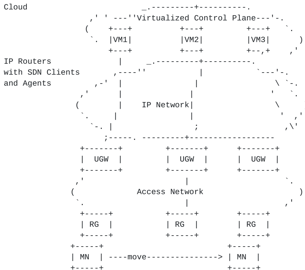
Figure 1: Architecture of DMM for Wi-Fi Protocol
