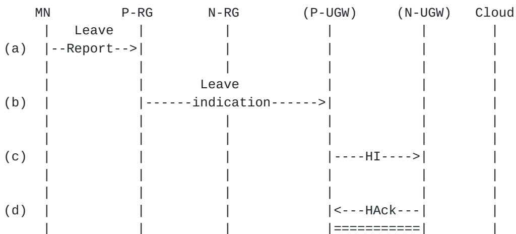
Figure 2: Predictive Handover
