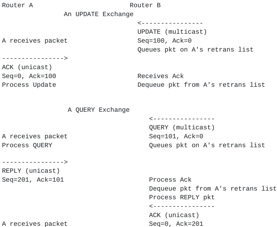
Figure 5 - Reliable Transfer on point-to-point links
