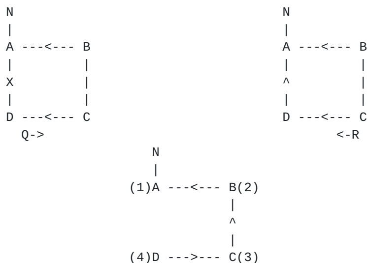
Figure 3 - Link between A and D fails
