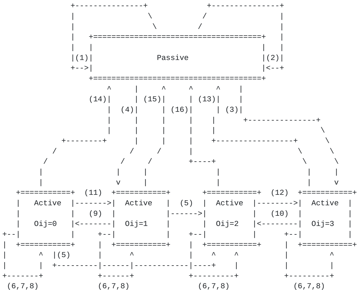
Figure 1 - DUAL Finite State Machine
