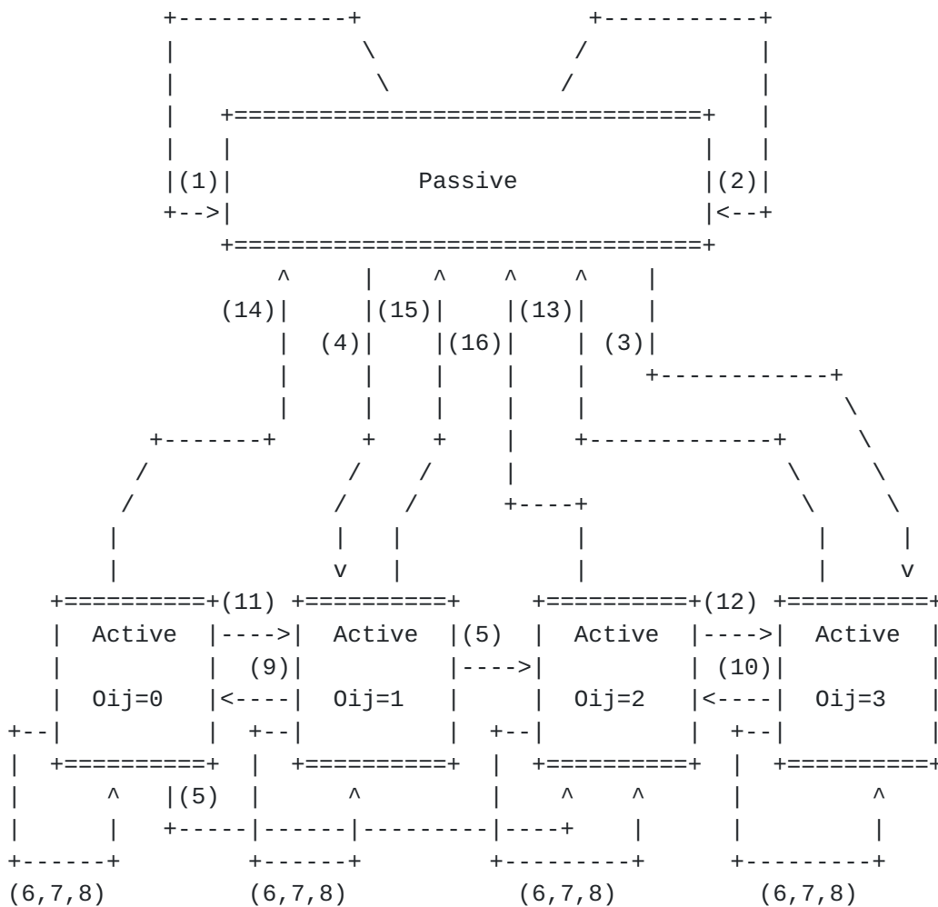
Figure 1 - DUAL Finite State Machine
