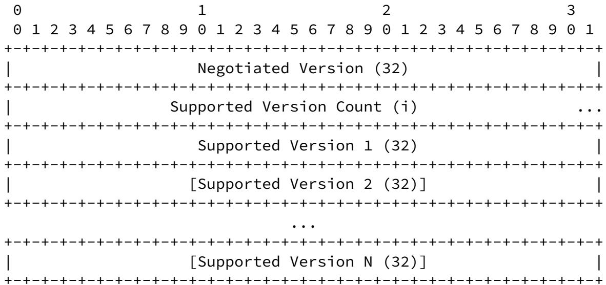
Figure 2: Server Transport Parameter Format
