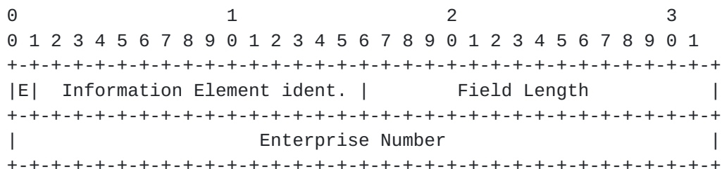
Figure 14: TinyIPFIX Template Header
