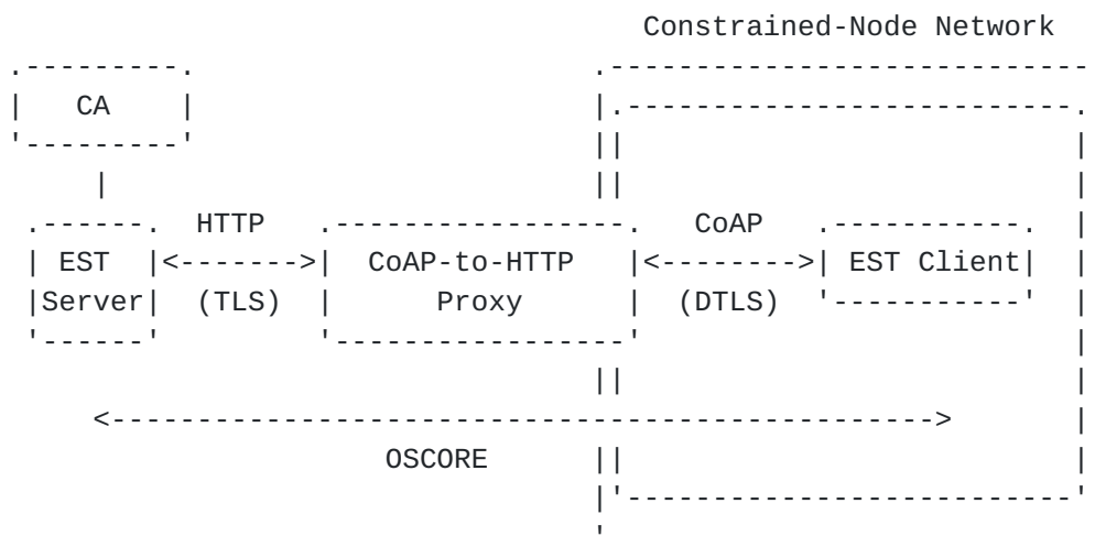
Figure 2: CoAP-to-HTTP proxy at the CoAP boundary.
