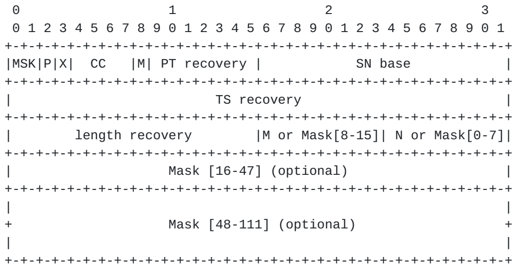
Figure 10: Format of the FEC header
