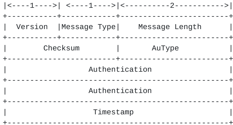
Figure 6: The Format of DLR Messages
