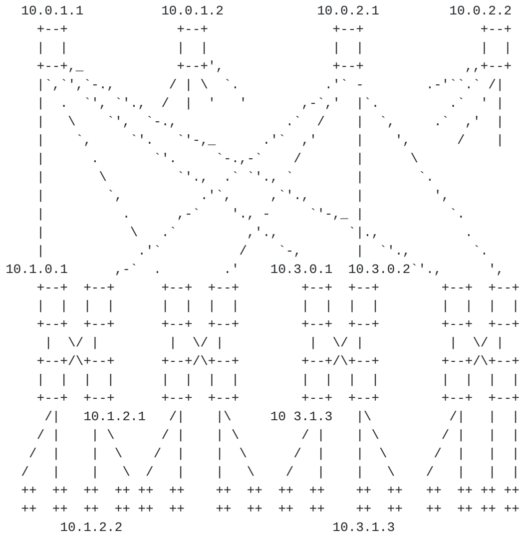
Figure 8: Fat-tree Network
