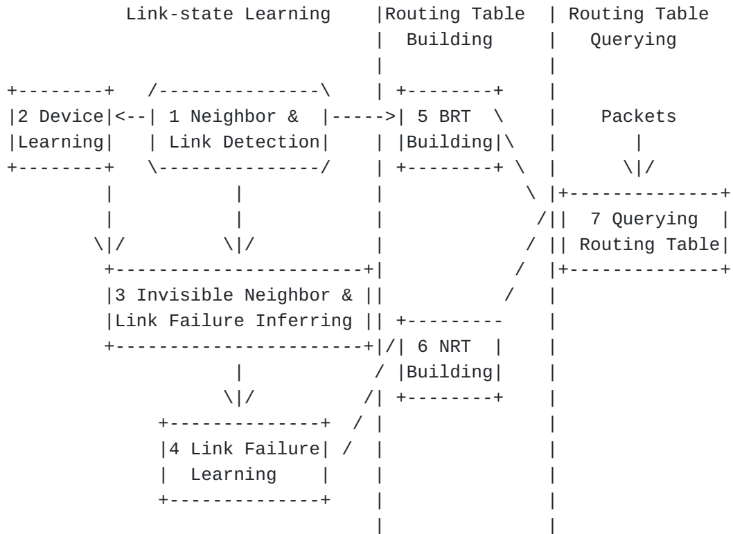
Figure 1: The FAR framework
