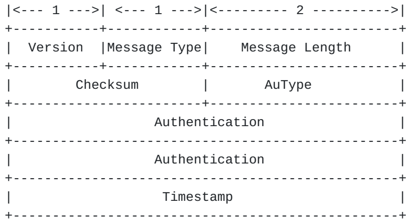
Figure 2: The format of FAR header
