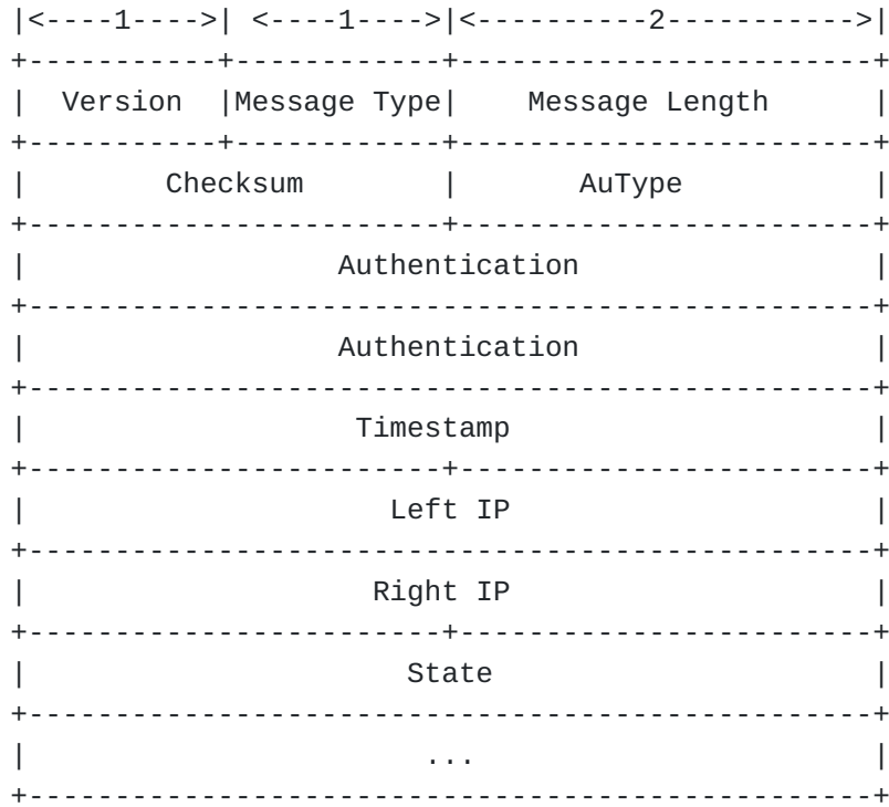
Figure 5: The Format of LFA Messages
