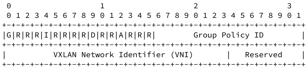
Figure 1: VXLAN-GBP Extension
