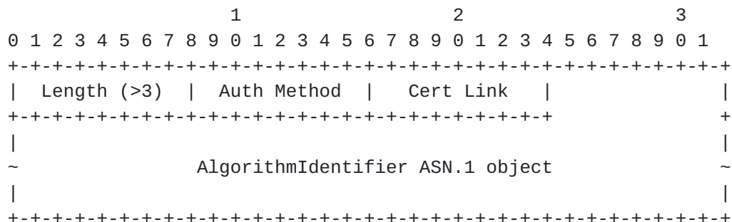
Figure 7: Supported Authentication Method
