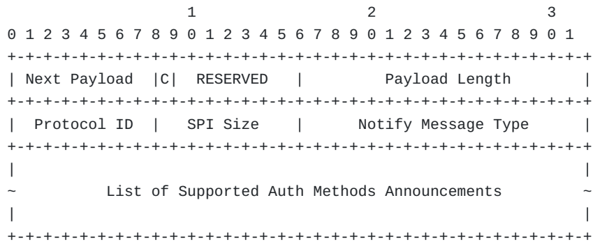
Figure 4: SUPPORTED_AUTH_METHODS Notify
