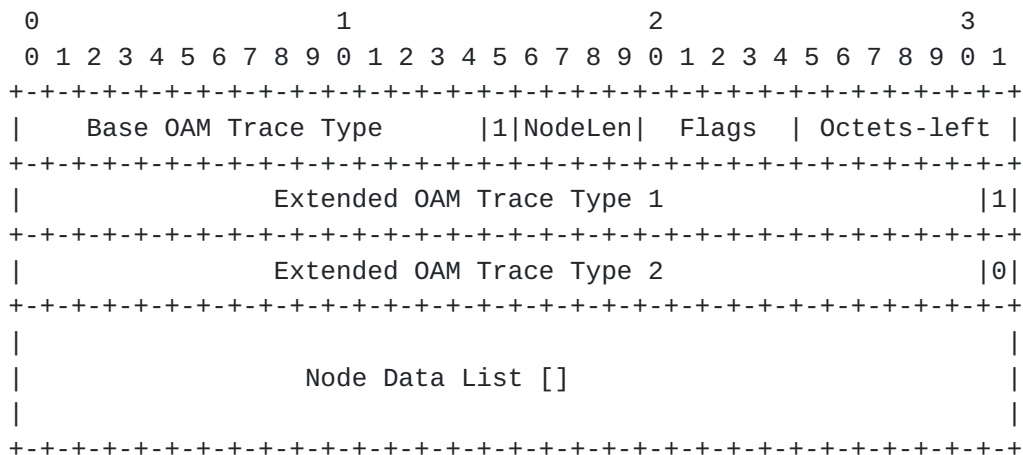
Figure 1: Extended OAM Trace Type Header Format
