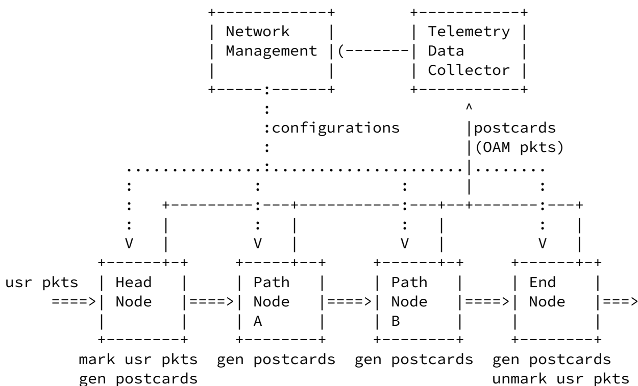
Figure 1: Architecture of PBT-M
