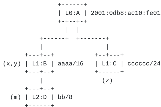
Figure 1: A Hierarchical Edge Network
