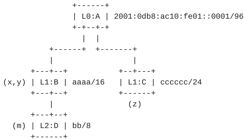
Figure 1: A Hierarchical Edge Network Example
