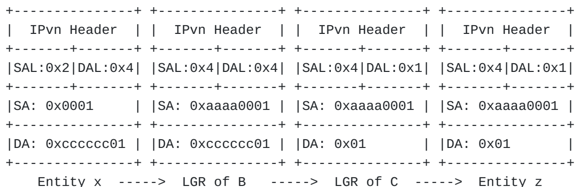
Figure 5: Forward to another network in the edge
