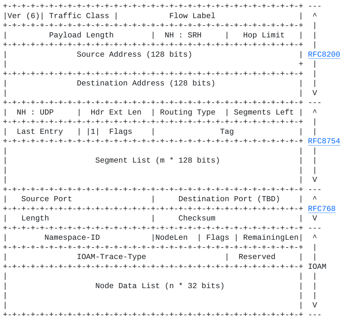
Figure 2: The active probing packet format
