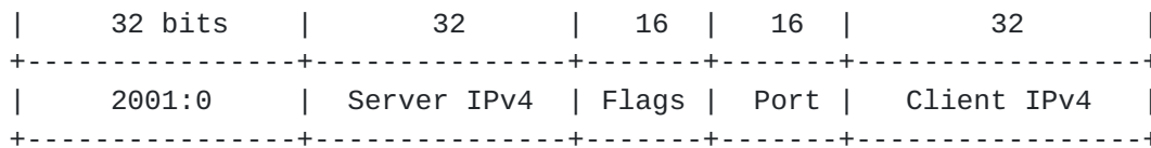
The Teredo address structure
