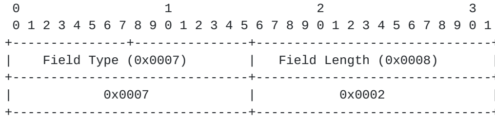
NTP Extension Field: I-Do - Example
