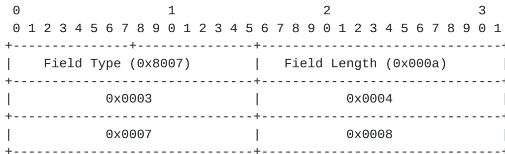
NTP Extension Field: I-Do Response - Example
