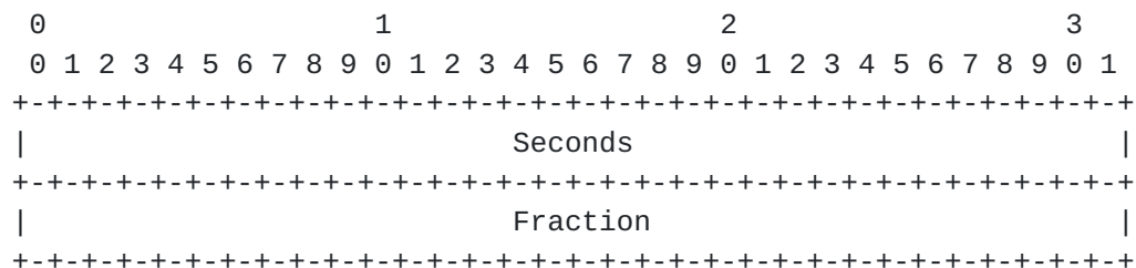
NTP Timestamp Format (32:32)
