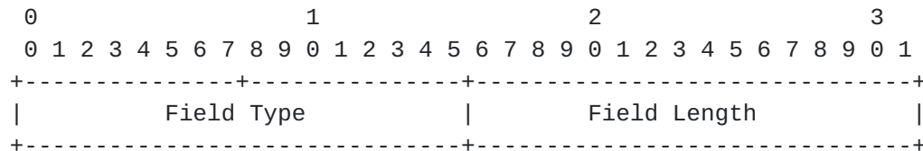
NTP Extension Field: Last Extension Field
