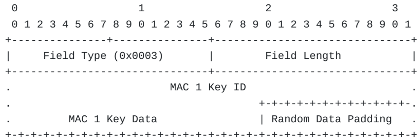
NTP Extension Field: MAC EF Format (Single MAC)
