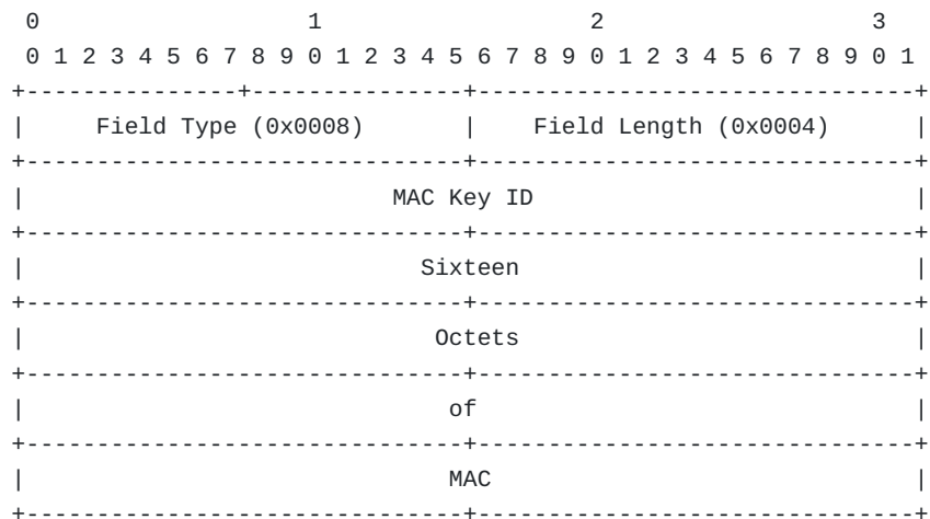
Example: NTP Extension Field: Last Extension Field, followed by a Legacy MAC
