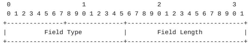
NTP Extension Field: Last Extension Field - LAST-EF
