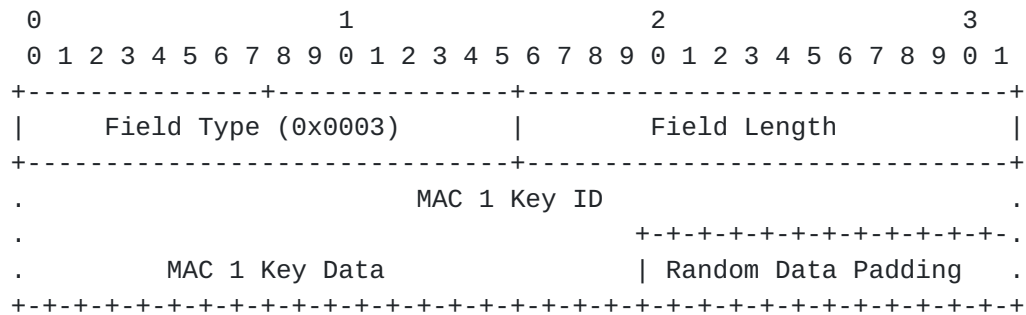
NTP Extension Field: MAC EF Format (Single MAC)
