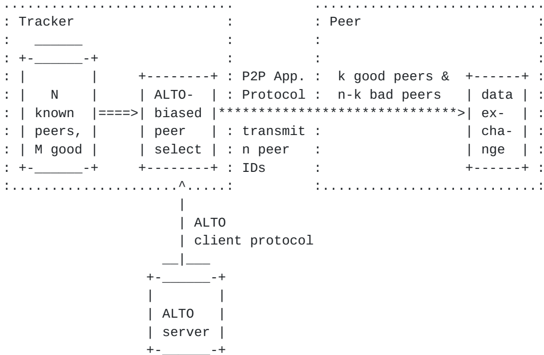
Figure 12: Tracker-based P2P Application with ALT0 client in tracker
