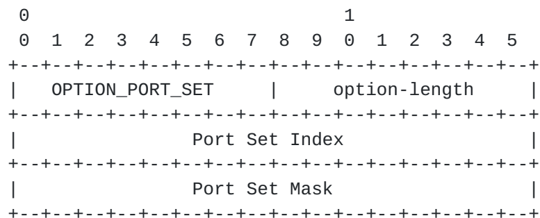
Figure 1 Port Set Option Format
