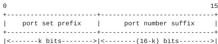
Figure 2 Bit Representation of a port number
