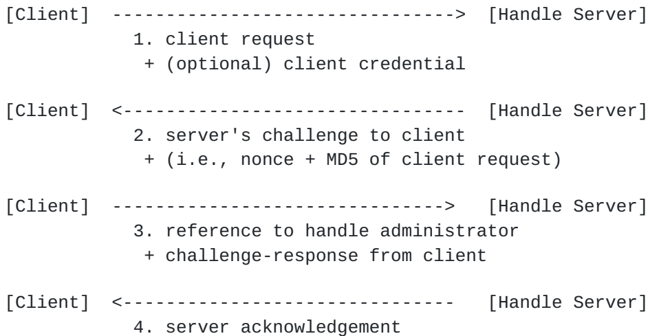
Figure 5.2: Handle system authentication process
