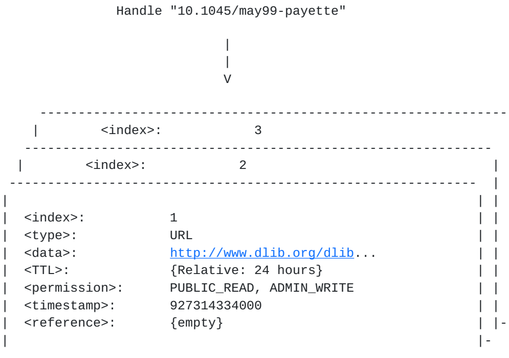
Figure 3.1: Handle "10.1045/may99-payette" and its set of values
