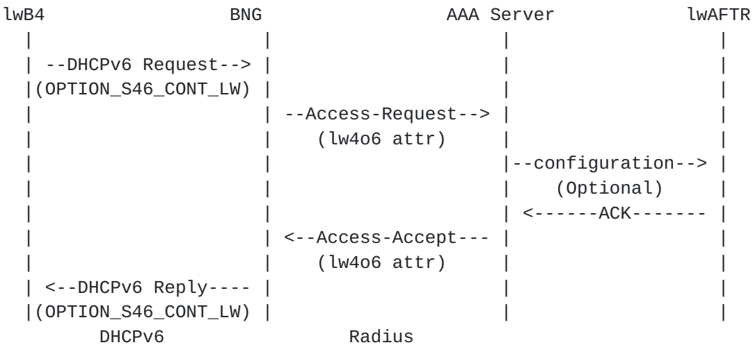
Figure 2: Lightweight 4over6 configuration process with RADIUS case 2
