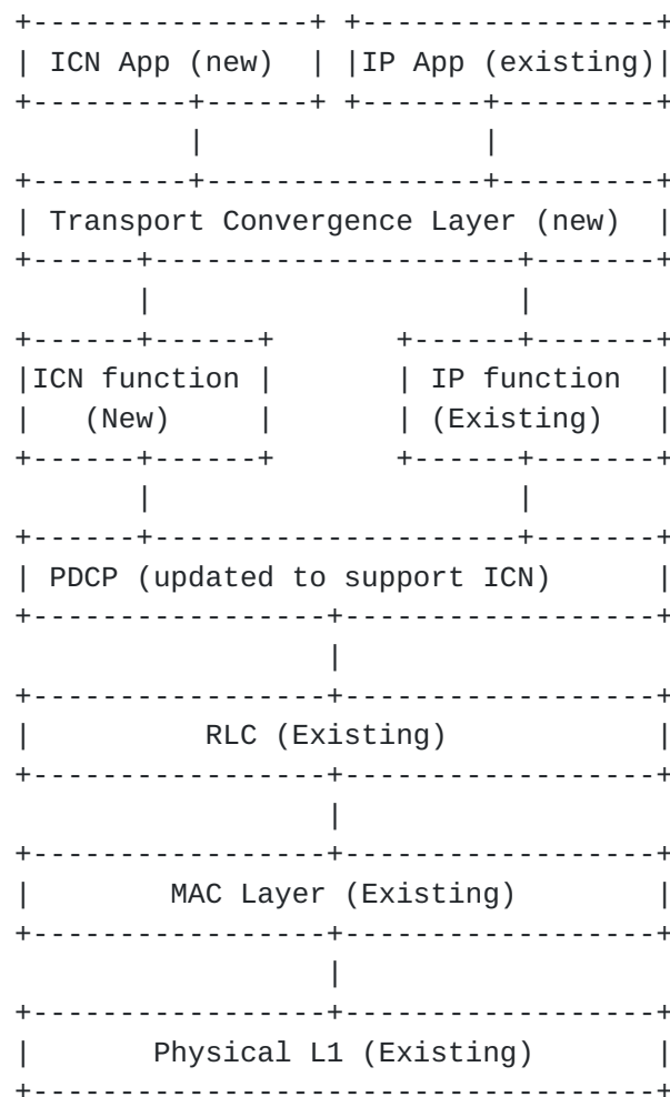
Fig. 7. Dual stack ICN protocol interactions
