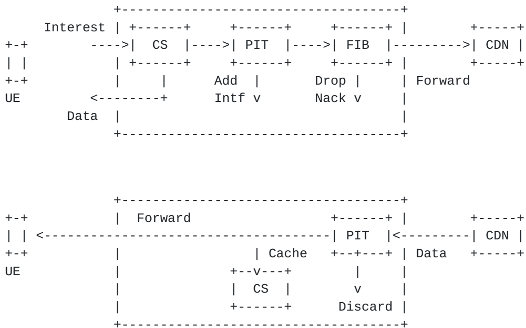
Fig. 3. ICN Interest, Data Packet and Forwarder
