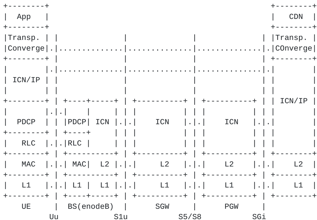
Fig. 8. Native ICN Deployment in UE
