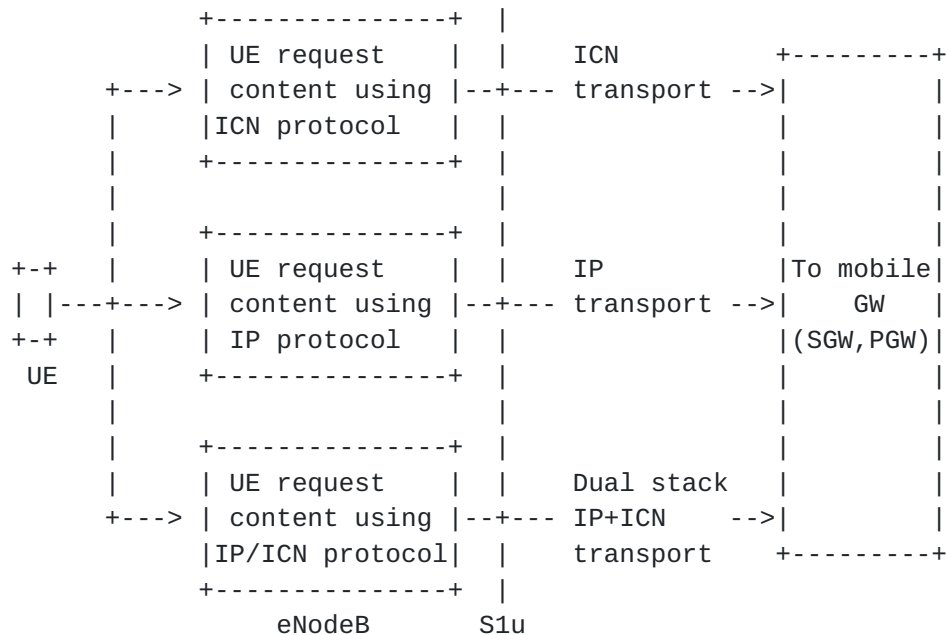
Fig. 9. Native ICN Deployment in eNodeB
