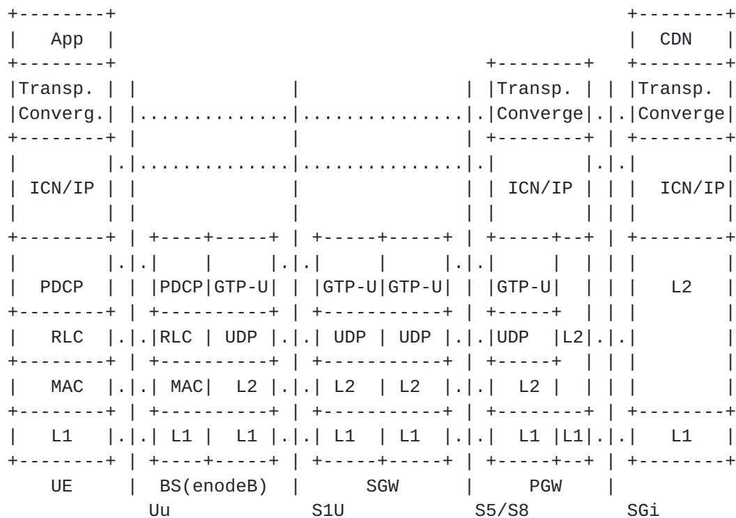
Fig. 6. Dual stack ICN Deployment in UE
