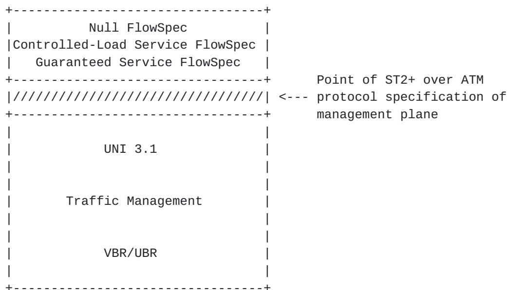
Fig. 2.3: Management plane protocol stack.
