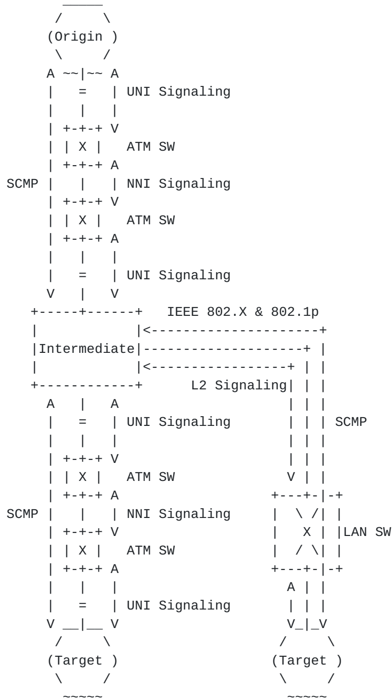
Fig. 2.6: Example of ST2+ SCMP interworking.
