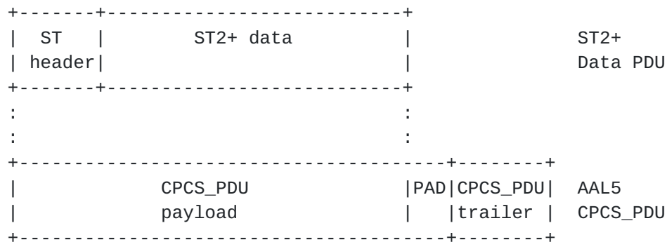
Fig. 4.1: Mapping of ST2+ data to AAL5 CPCS_PDU payload.
