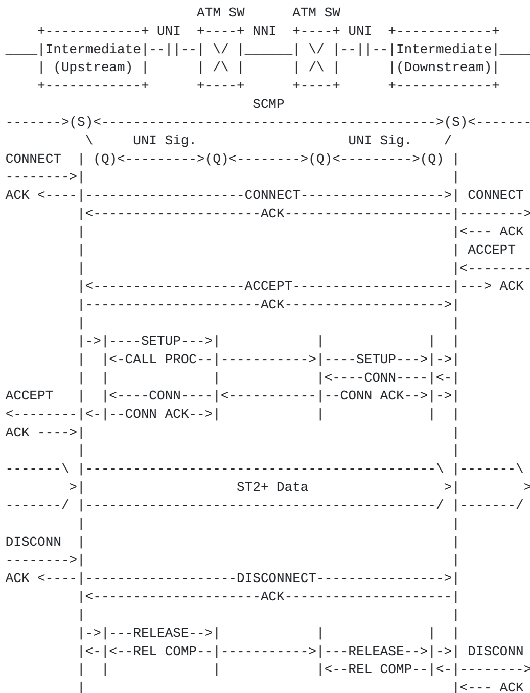
Fig. 2.5: Example of ST2+ SCMP and UNI 3.1 signaling message flows.
