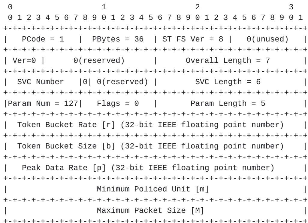
Fig. 3.1: Format of ST FlowSpec for Controlled-Load Service.
