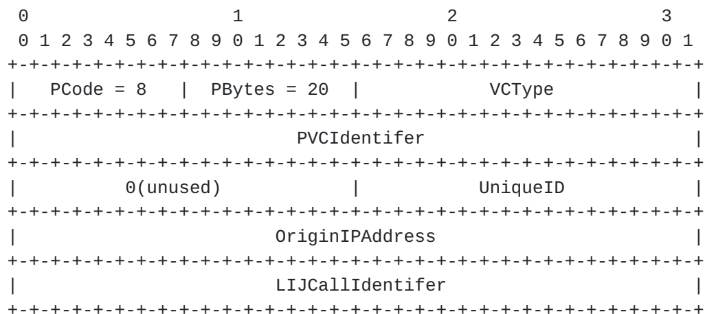
Fig. 3.2: Format of VC-type common SCMP element.
