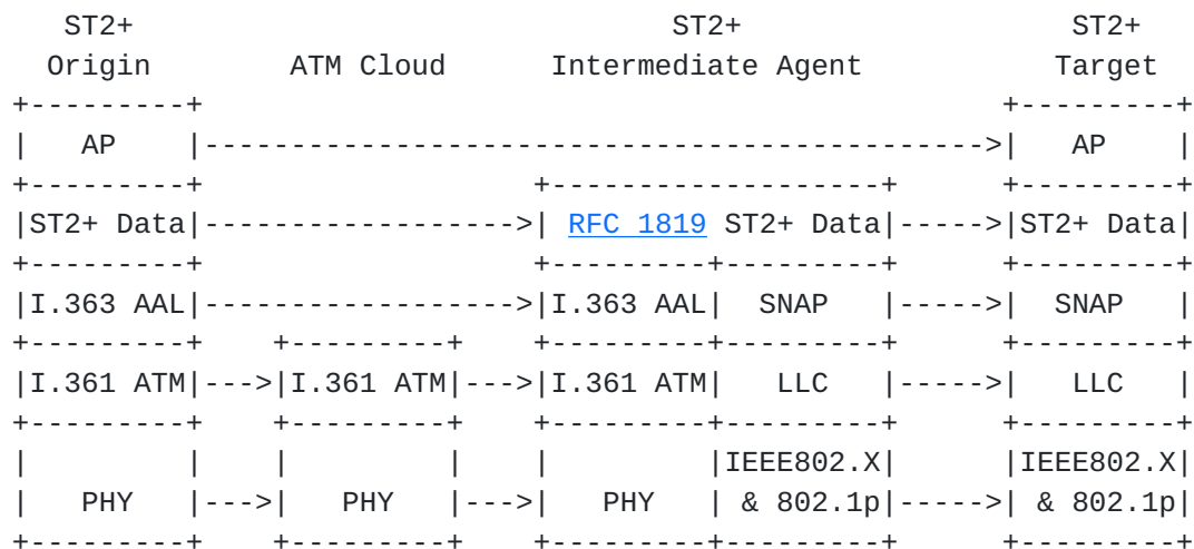
Fig. 2.2: Example of interworking from an ATM network to an IEEE 802.X LAN.
