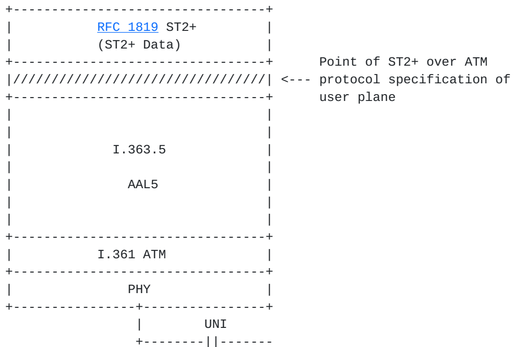
Fig. 2.1: User plane protocol stack.
