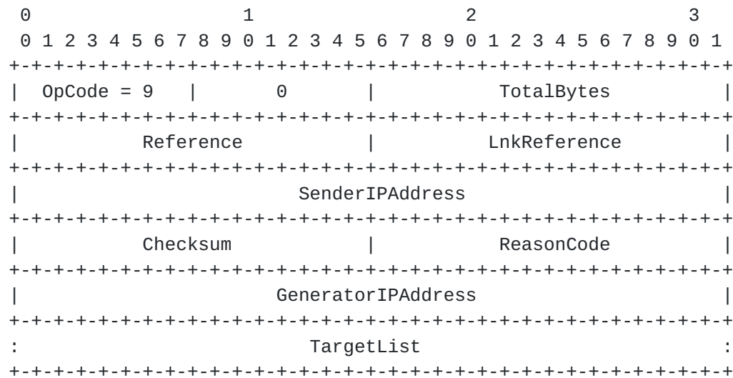
Fig. 3.3: JOIN-REJECT Control Message.
