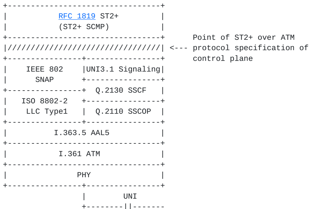
Fig. 2.4: Control plane protocol stack.
