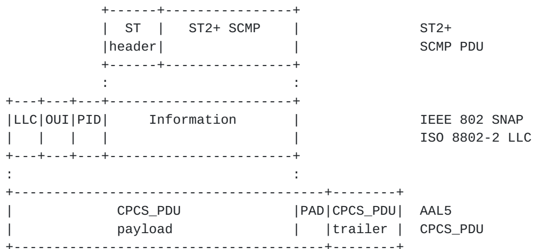
Fig. 6.1: Mapping of ST2+ SCMP PDU to AAL5 CPCS_PDU payload.
