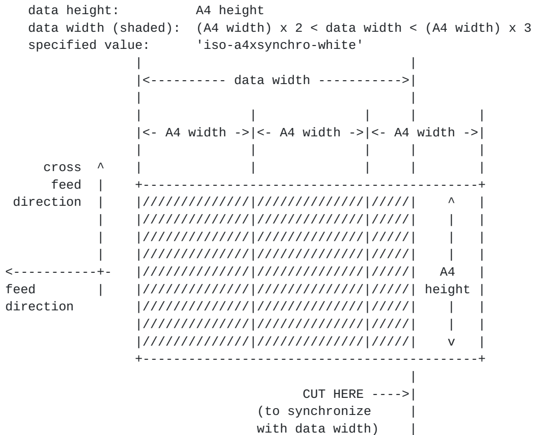
Example 4: "Synchro-Cut", a device cutting the fixed size paper in synchronization with the data
