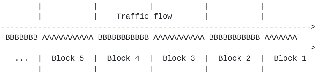
Figure 2: Traffic coloring
