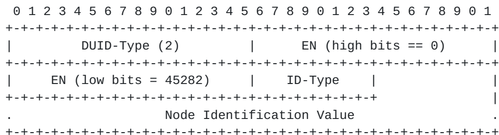
Figure 29: DUID-EN for OMNI Format
