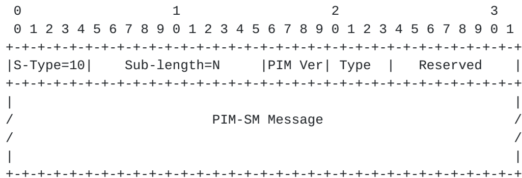
Figure 24: PIM-SM Message Option Format
