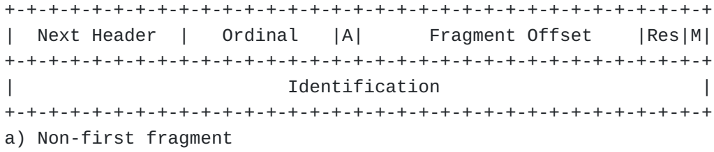
Figure 4: IPv6 Fragment Header Reserved Fields Redefined
