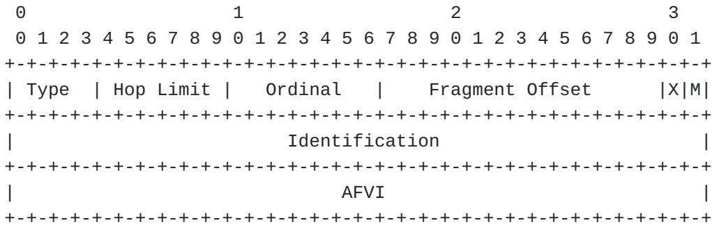
Figure 7: OMNI Compressed Header - Type 2 (OCH-2)
