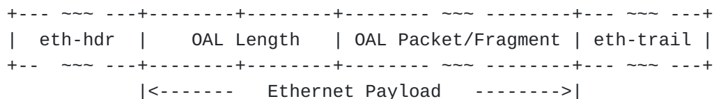
Figure 10: OMNI Ethernet Frame Format
