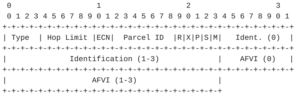
Figure 6: OMNI Compressed Header - Type 1 (OCH-1)
