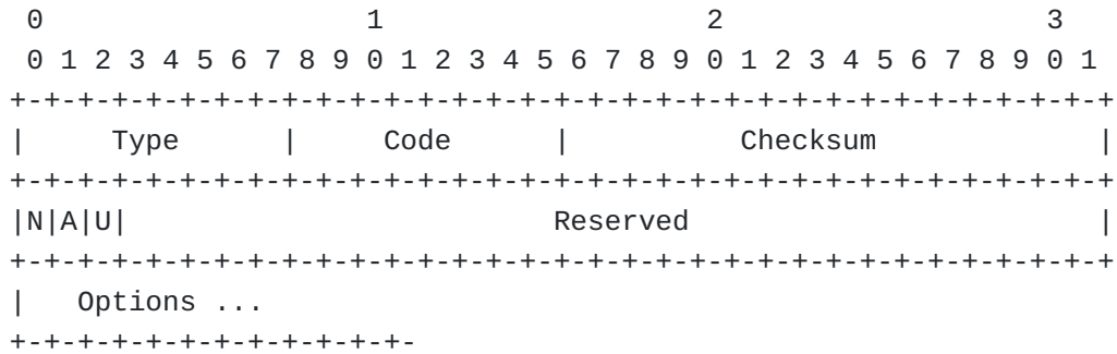
Figure 36: OMNI-Enhanced Router Solicitation Message Format
