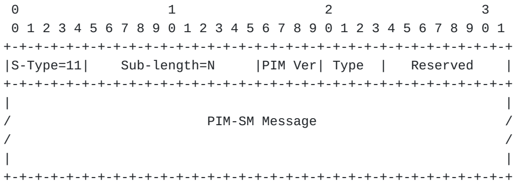
Figure 26: PIM-SM Message Option Format
