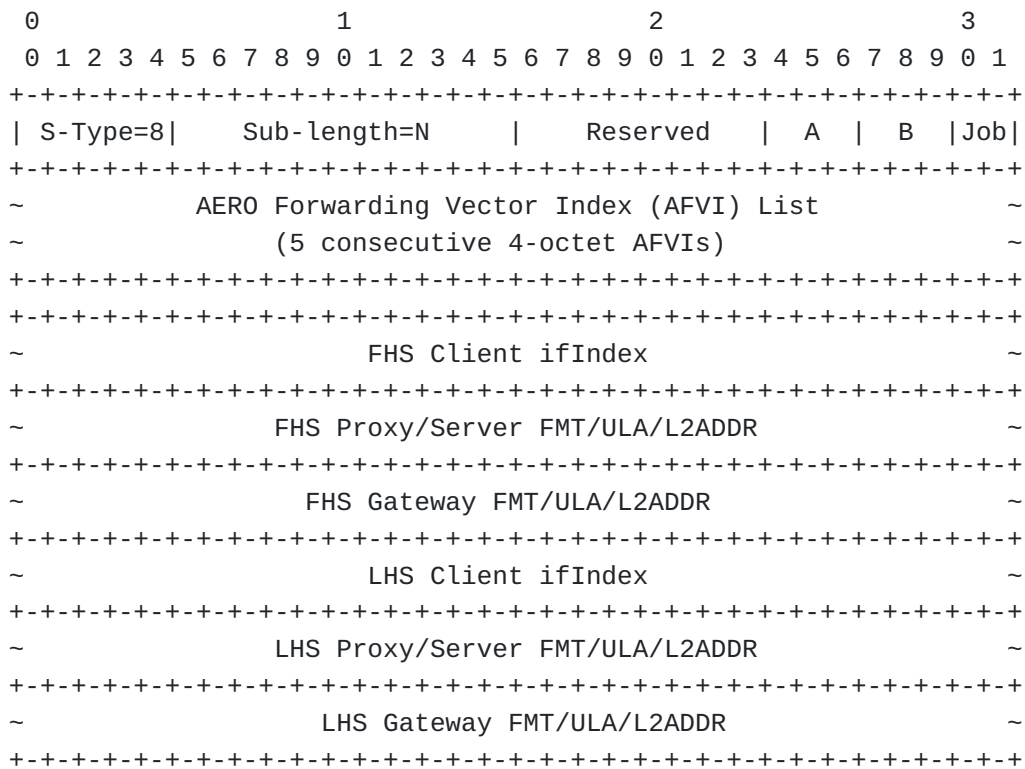
Figure 23: AERO Forwarding Parameters
