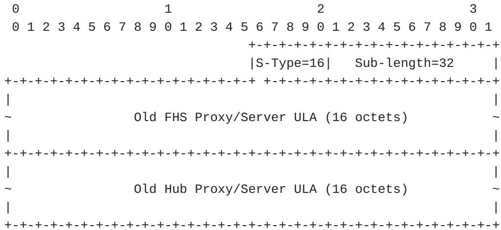
Figure 32: Proxy/Server Departure
