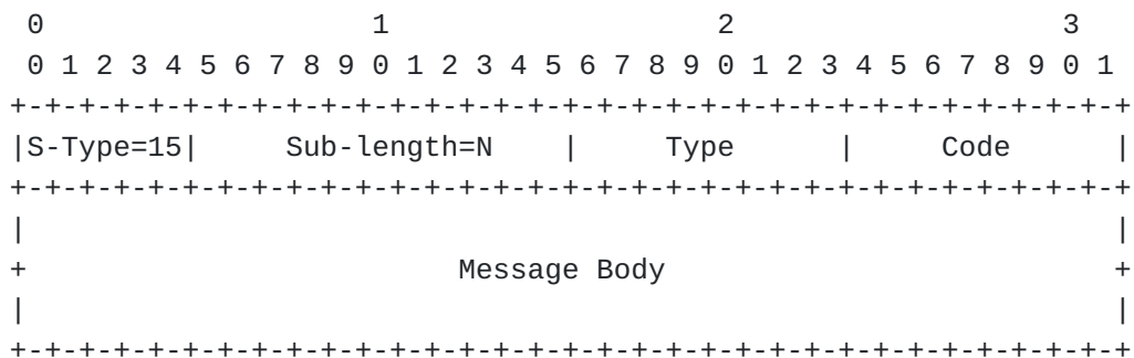
Figure 31: ICMPv6 Error
