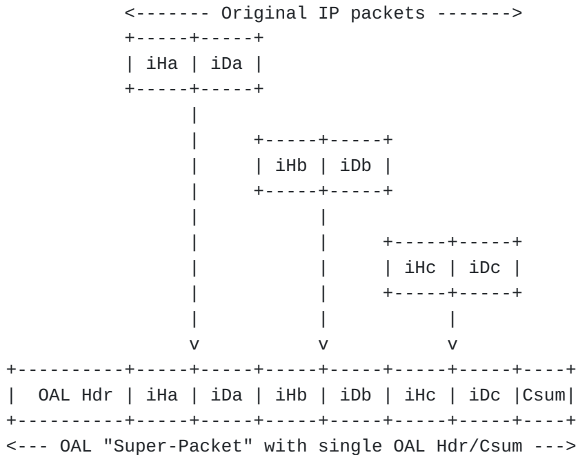
Figure 9: OAL Super-Packet Format
