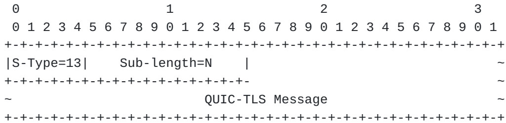
Figure 28: QUIC-TLS Message
