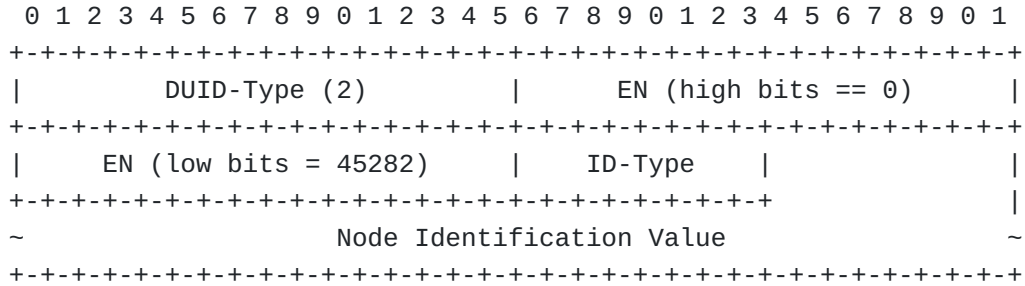
Figure 17: DUID-EN for OMNI Format
