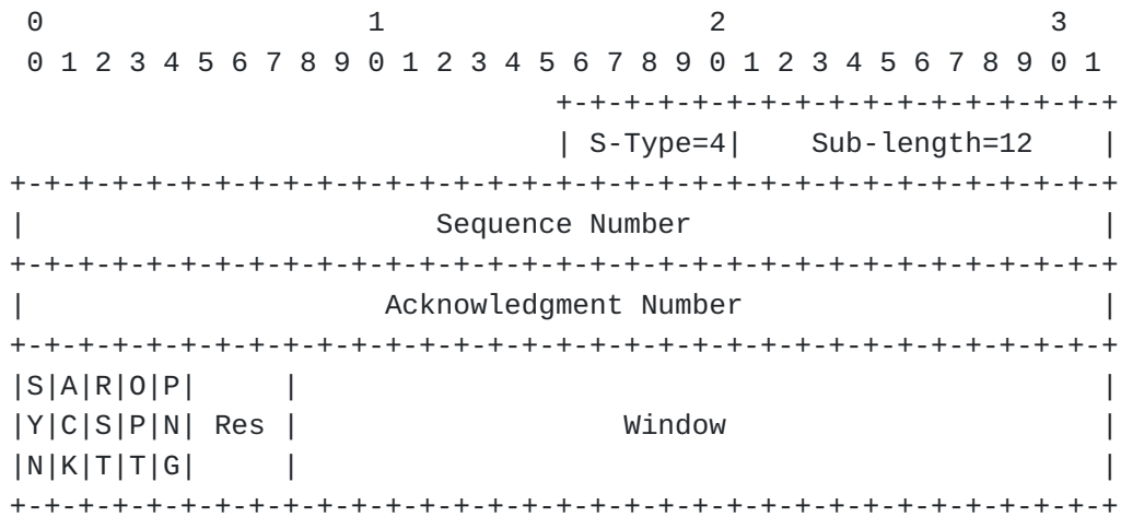
Figure 19: Window Synchronization
