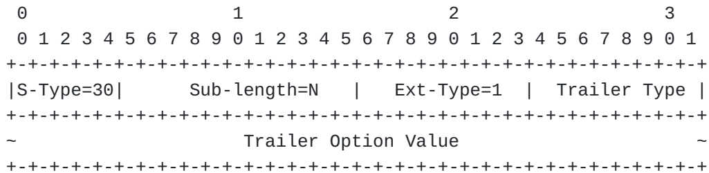
Figure 35: RFC6081 Trailer Extension Option (Extension-Type 1)
