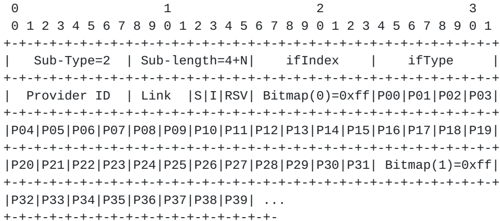
Figure 8: ifIndex-tuple (Type 1)
