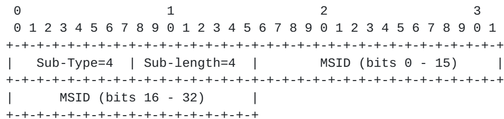
Figure 11: MS-Register Sub-option
