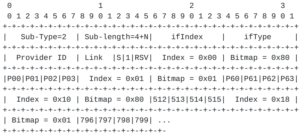
Figure 18: Example 3: Indexed Encoding
