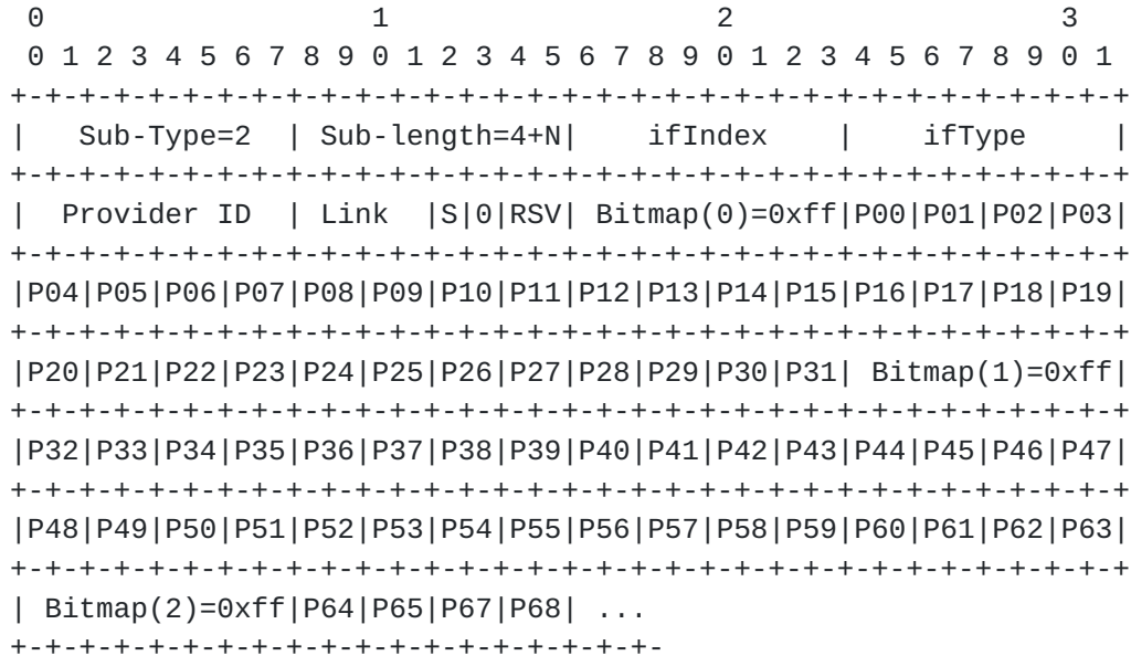
Figure 16: Example 1: Dense Simplex Encoding
