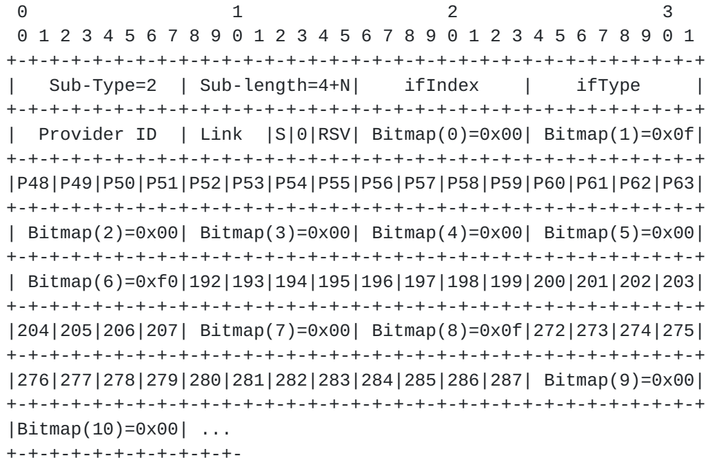
Figure 17: Example 2: Sparse Simplex Encoding
