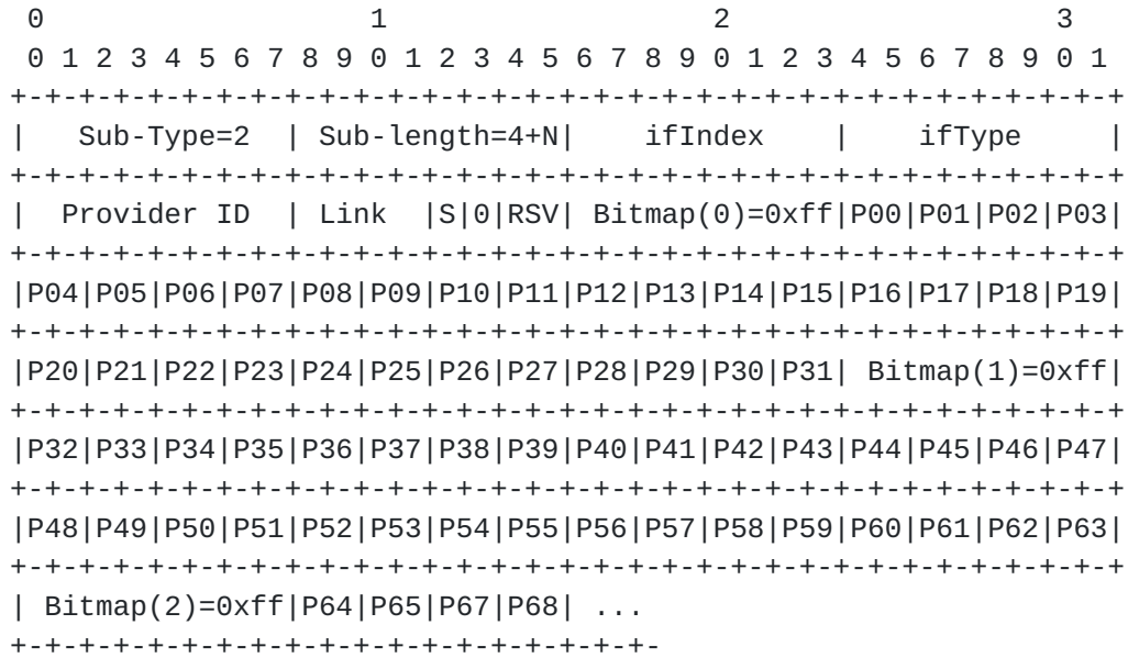
Figure 16: Example 1: Dense Simplex Encoding
