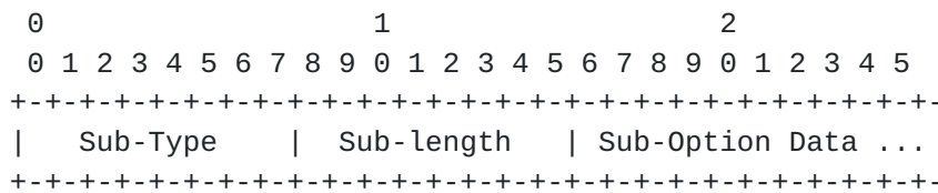
Figure 4: Sub-Option Format
