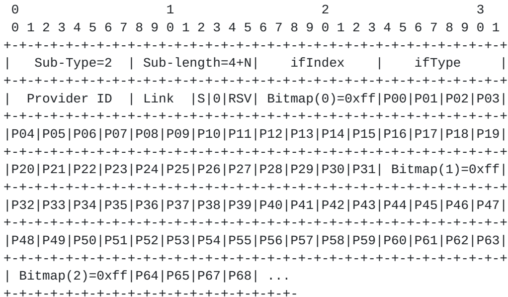
Figure 17: Example 1: Dense Simplex Encoding
