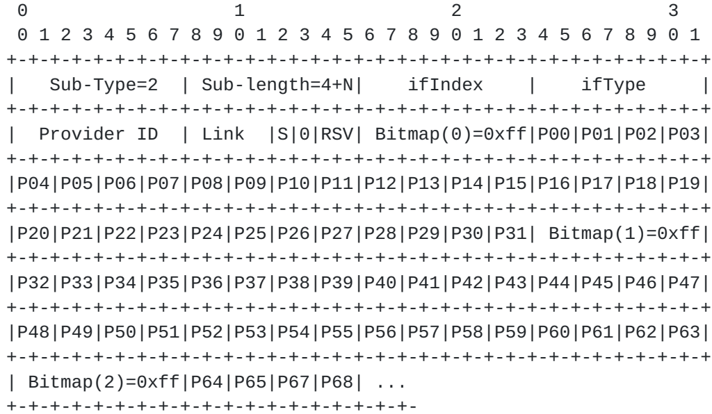
Figure 18: Example 1: Dense Simplex Encoding
