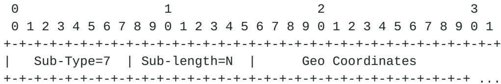
Figure 14: Geo Coordinates Sub-option
