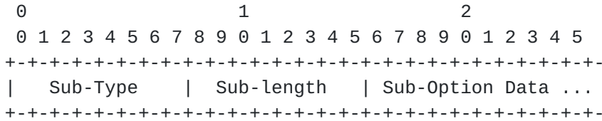
Figure 4: Sub-Option Format
