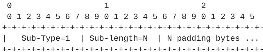
Figure 7: PadN
