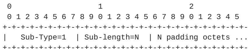
Figure 7: PadN
