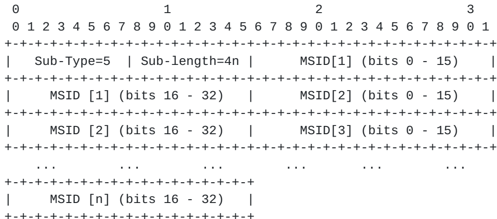
Figure 12: MS-Release Sub-option
