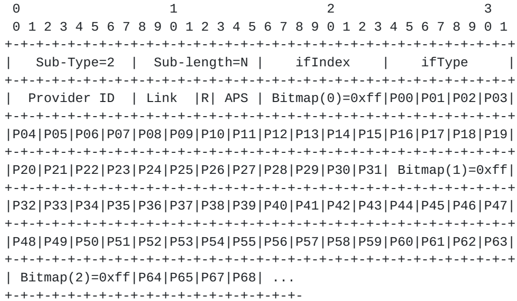
Figure 18: Example 1: Dense Simplex Encoding
