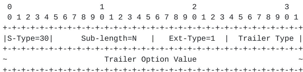
Figure 22: RFC6081 UDP/IP Trailer Option (Extension-Type 1)
