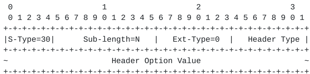
Figure 21: RFC4380 UDP/IP Header Option (Extension-Type 0)
