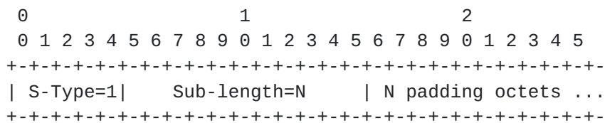
Figure 9: PadN
