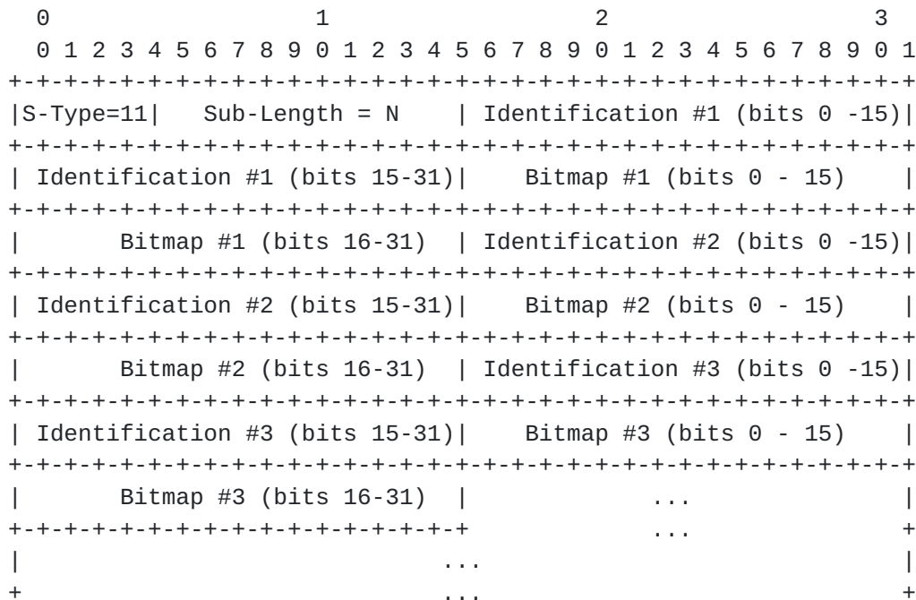
Figure 20: Fragmentation Report
