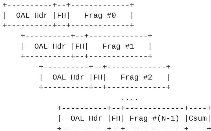
a) OAL fragments after fragmentation (FH = Fragment Header; Csum appears only in final fragment)
