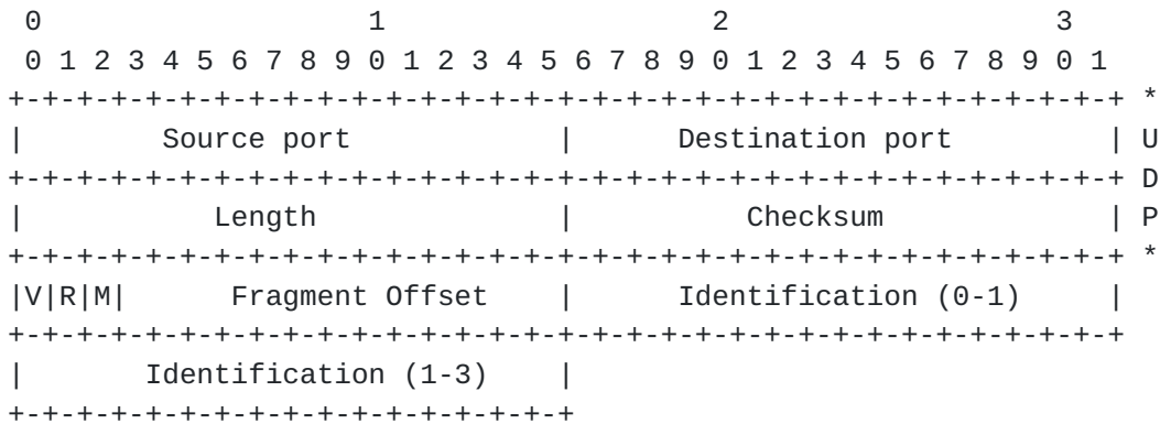
Figure 8: OMNI Compressed Header - Type 1 (OCH-1)
