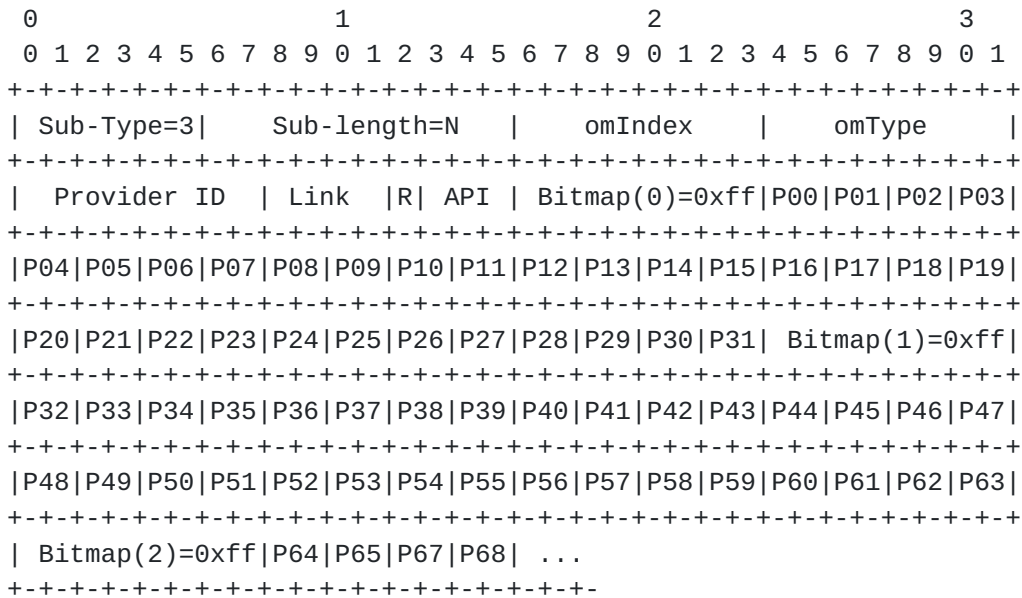
Figure 39: Example 1: Dense Simplex Encoding
