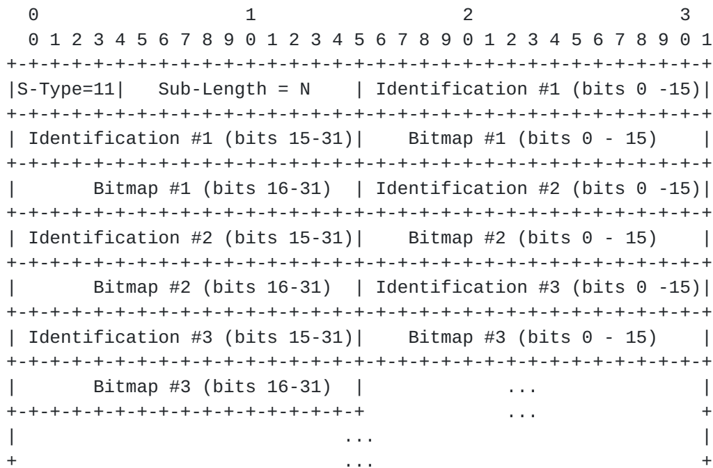
Figure 25: Fragmentation Report
