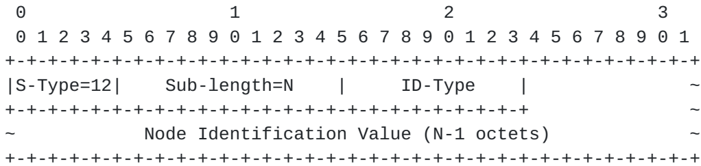
Figure 27: Node Identification
