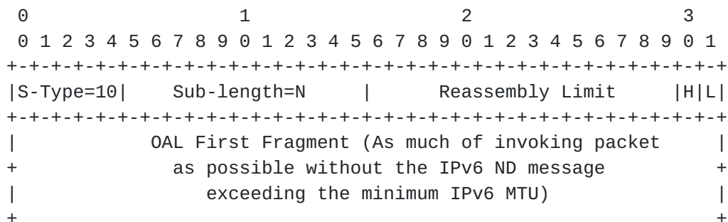
Figure 24: Reassembly Limit
