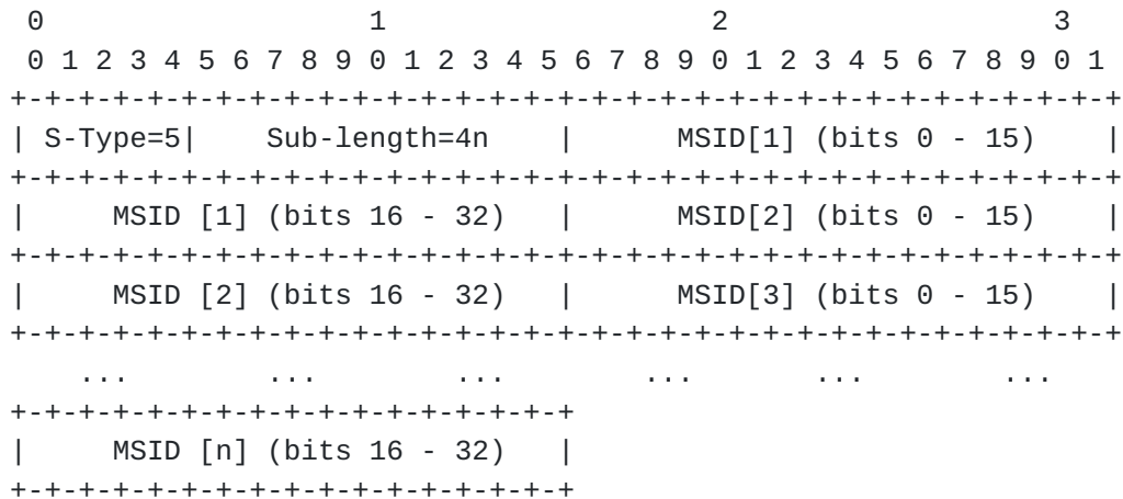
Figure 19: MS-Register Sub-option
