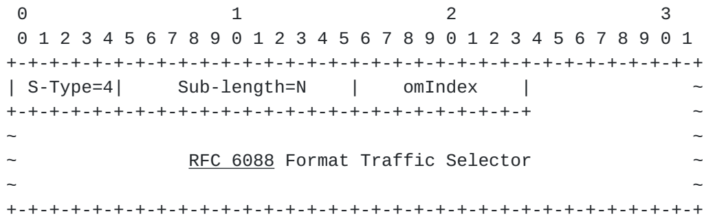
Figure 18: Traffic Selector
