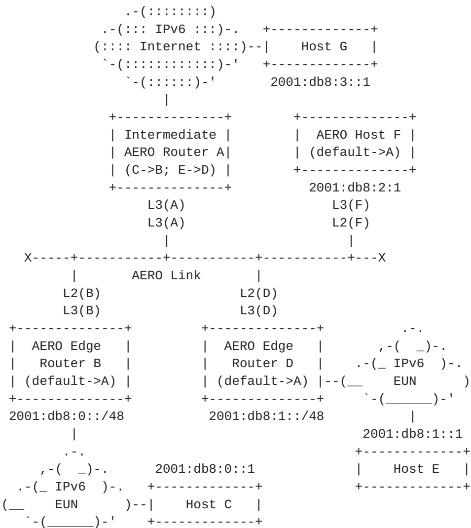
Figure 3: AERO Reference Operational Scenario
