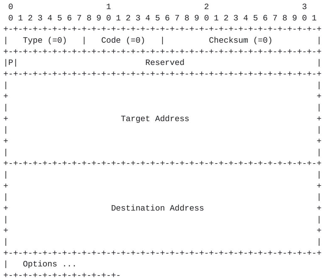
Figure 4: AERO Redirection Message Format
