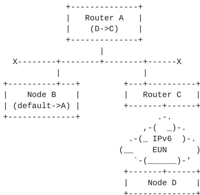
Figure 1: Classical Multi-Access Link Redirection
