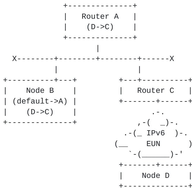
Figure 2: More-Specific Routes Following Redirection
