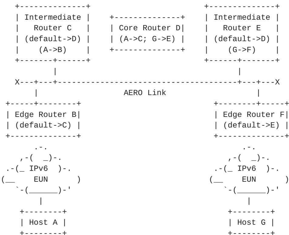
Figure 6: Multiple Intermediate Routers
