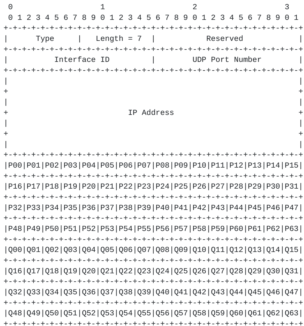
Figure 7: ATN/IPS Extended S/TLLAO Format
